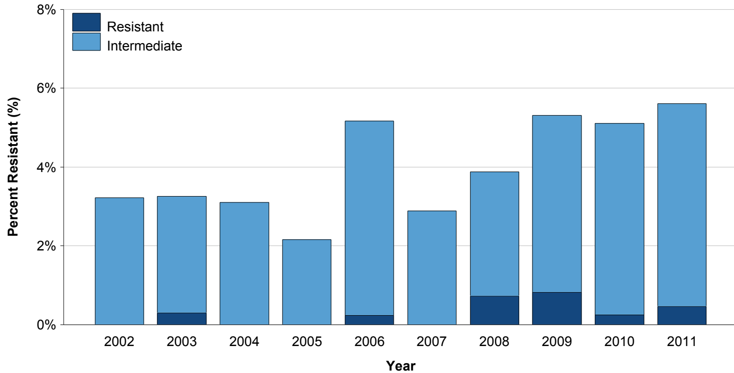
Penicillin Resistance S. pneumoniae isolates from respiratory sites, non-meningitis breakpoints, 2002-2011
