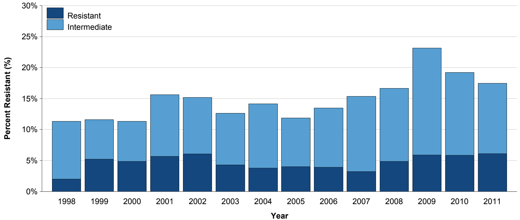
Penicillin Resistance S. pneumoniae isolates from sterile sites, meningitis breakpoints, 1998-2011
